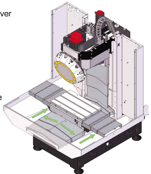
Telescopic covers are applied on all axes
