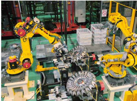
Automatic assembly line of ATC unit
