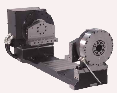
DDR-TiB/DDR-THPiB The trunnion unit that allows easy creation of machining fixture making the most of the ROBODRILL's machining stroke. Clamping torque: 1100N·m
