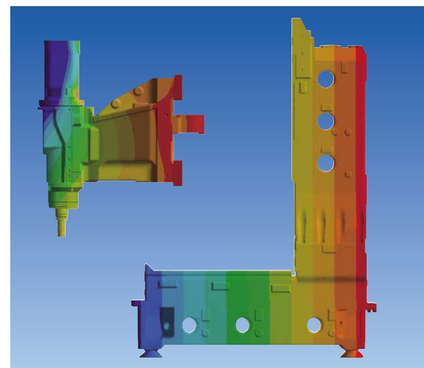
Extending straightly and easy to compensate
