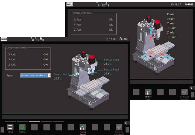
Thermal displacement compensation function
