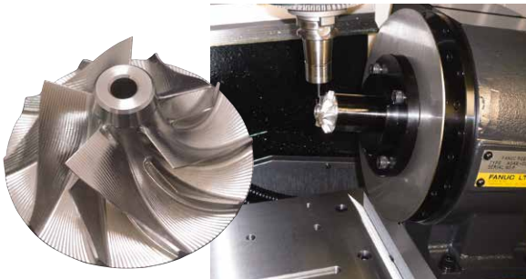
High-speed machining of impellers using a 1-axis DD motor rotary table DDR/B
