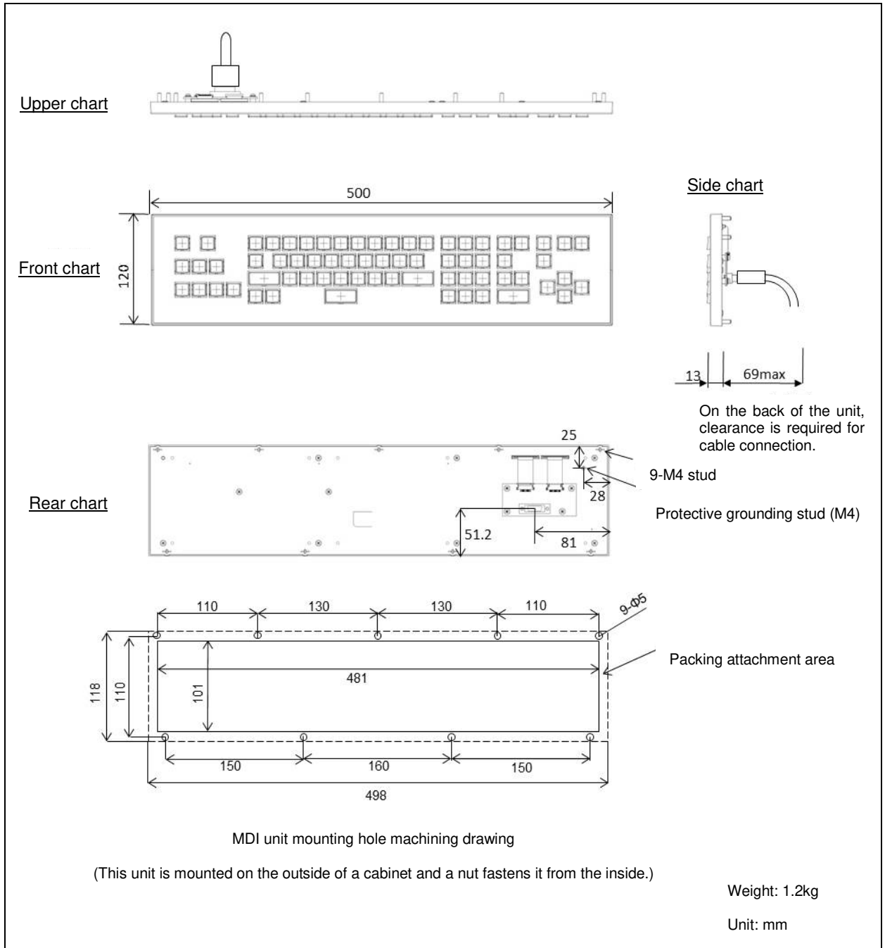
Fig. U15 MDI unit (QWERTY TYPE C, 120x500mm) ①⑥
