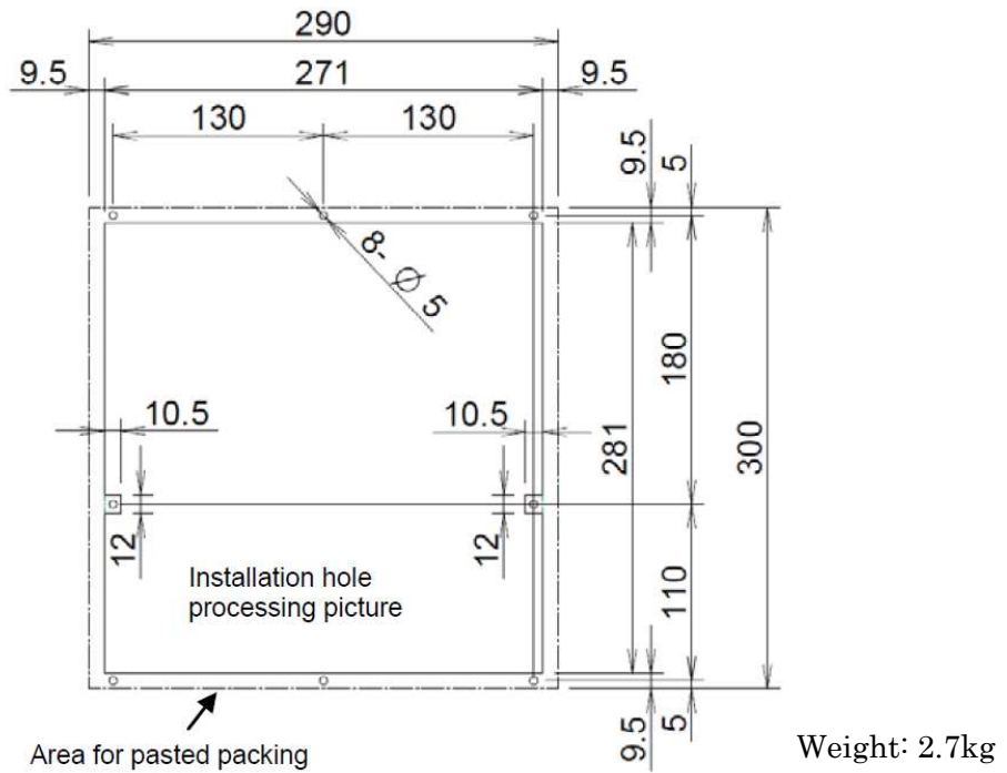
Fig. U17 10.4" LCD/MDI unit B(Vertical) 08
